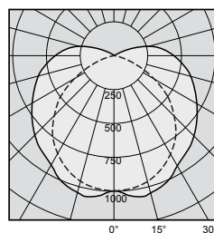
FL98016 - Viking LED Batten 4K Mains ULOR: 10% DLOR: 90%
