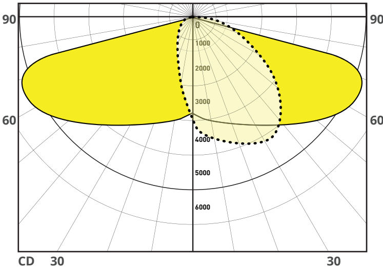
FLFL180 - OPTILUM LED FLOODLIGHT — C0 .....C90
